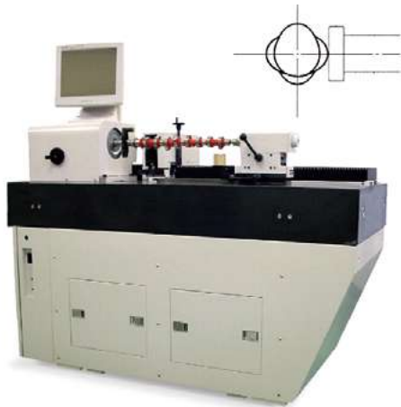
カム形状測定機 Cam Profile Digital Measuring Equipment
